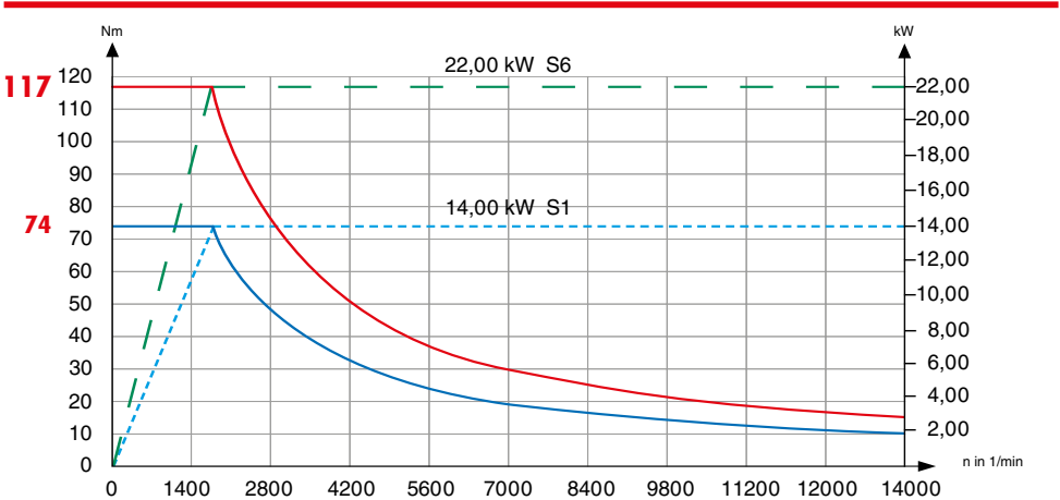
SK40/BT40, CELOX 14000 1/min, 117 Nm, 22,00 kW
