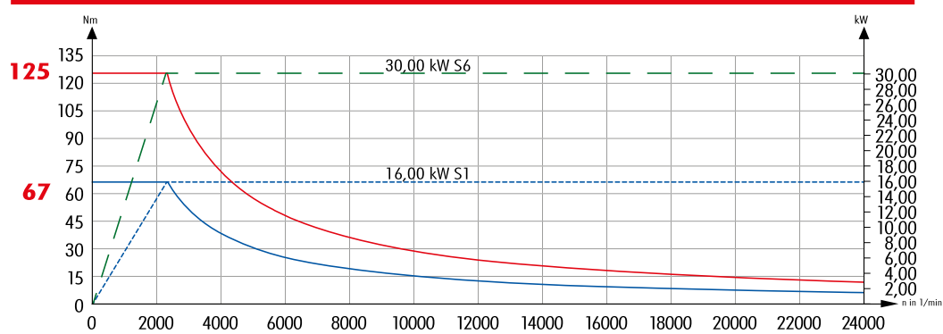
HSK A63, CELOX 24000 1/min, 125 Nm, 30,00 kW
